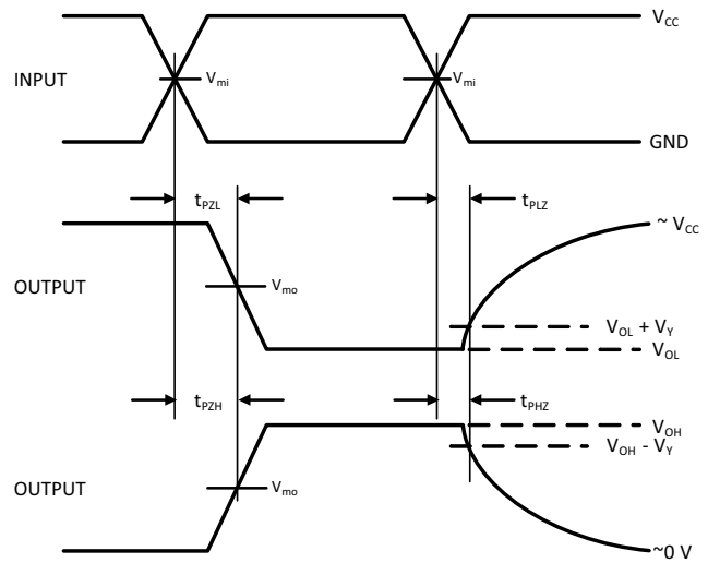
Figure 3. Switching Waveforms
