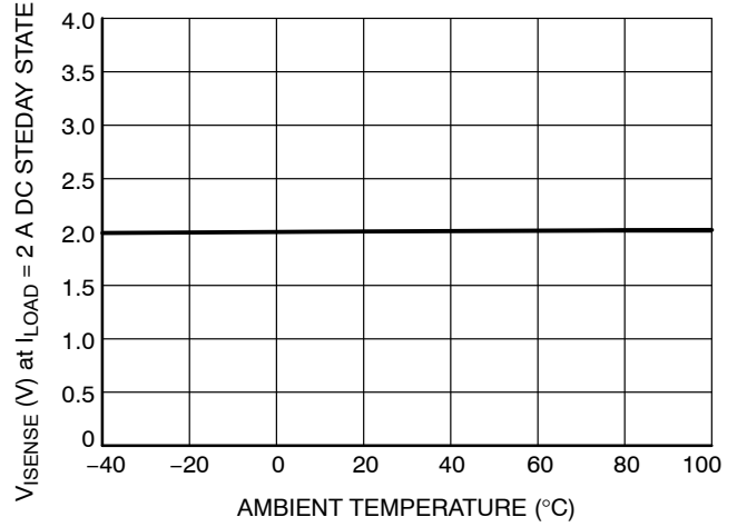
Figure 11. V_{SENSE} vs. Ambient Temperature
