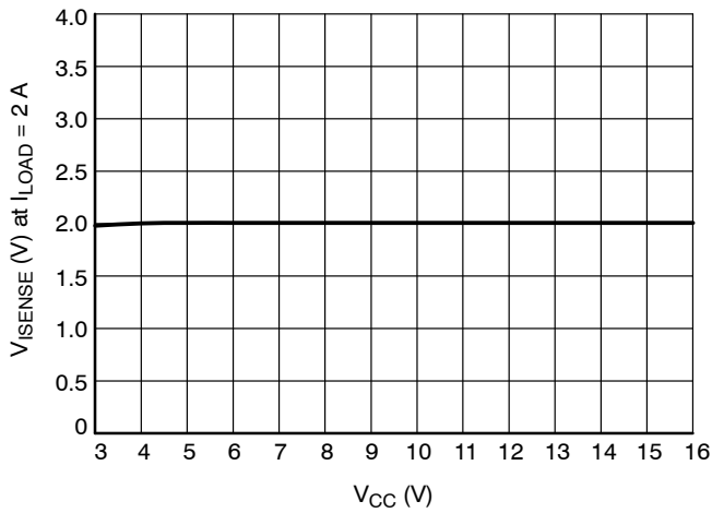
Figure 12. V_{SENSE} vs. V_{CC}
