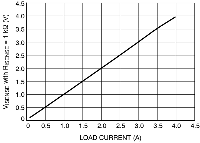
Figure 10. V_{SENSE} vs. Load Current
