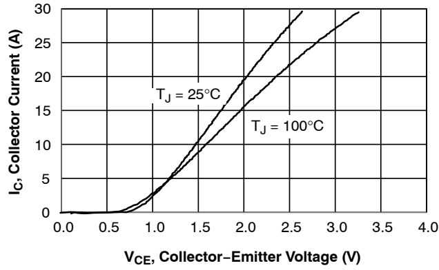
Figure 4. V_{CE} versus I_C for Different Temperatures ( V_{DD} = 15 V)
