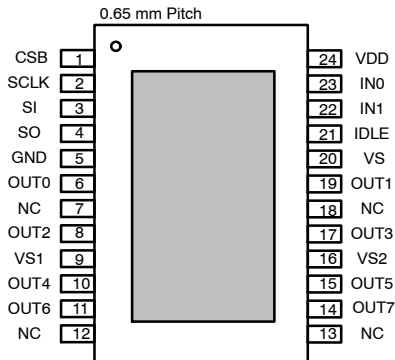
Figure 3. Pin-out
