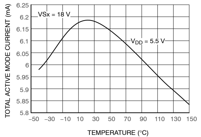
Figure 14. Total Active Mode Current vs. Temperature
