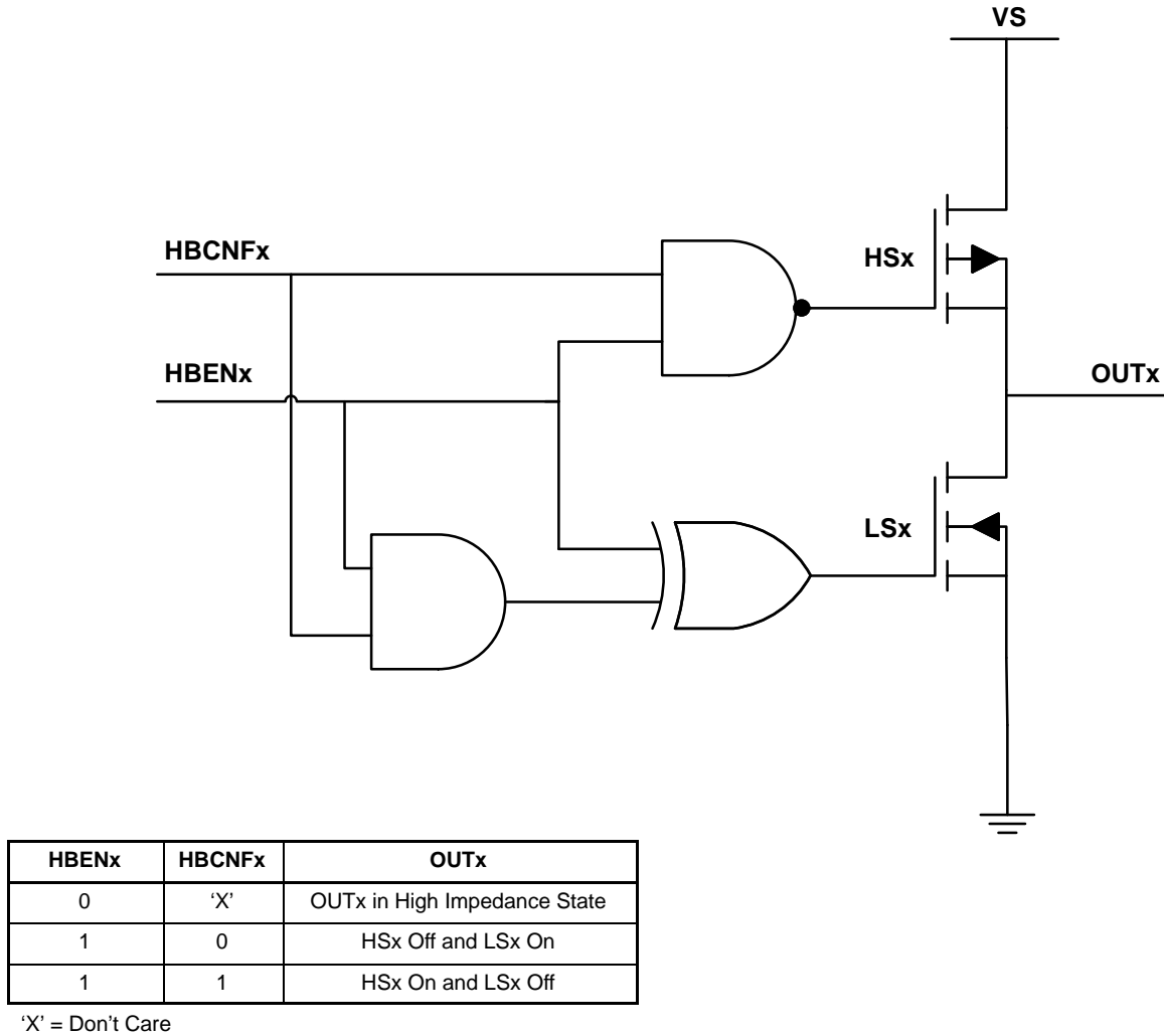
Figure 15. Bridge Control Logic
