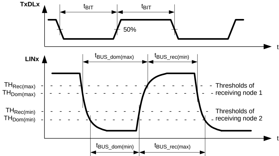
Figure 24. Definition of LINx Duty Cycle Parameters
