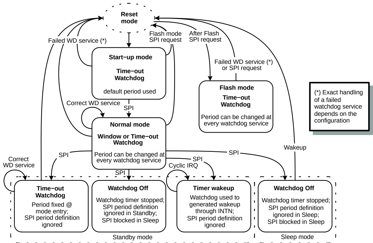
Figure 14. Watchdog Modes
