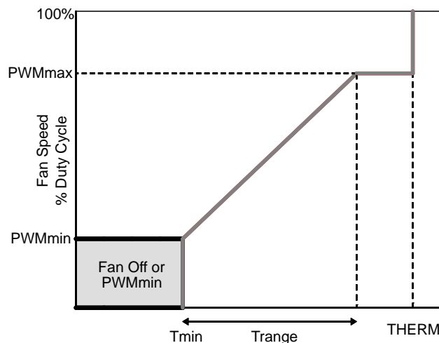
Figure 11. PWM Control Curve in Tmin/Trange Mode
