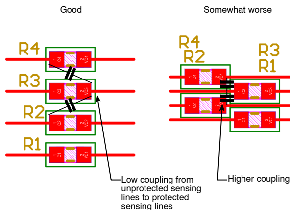
Figure 11. Care Must be Taken to Minimise the Coupling between Nets Before and Nets After the Cell-Sensing Filter Resistor. Left: Low Coupling; Right: Higher Coupling.
