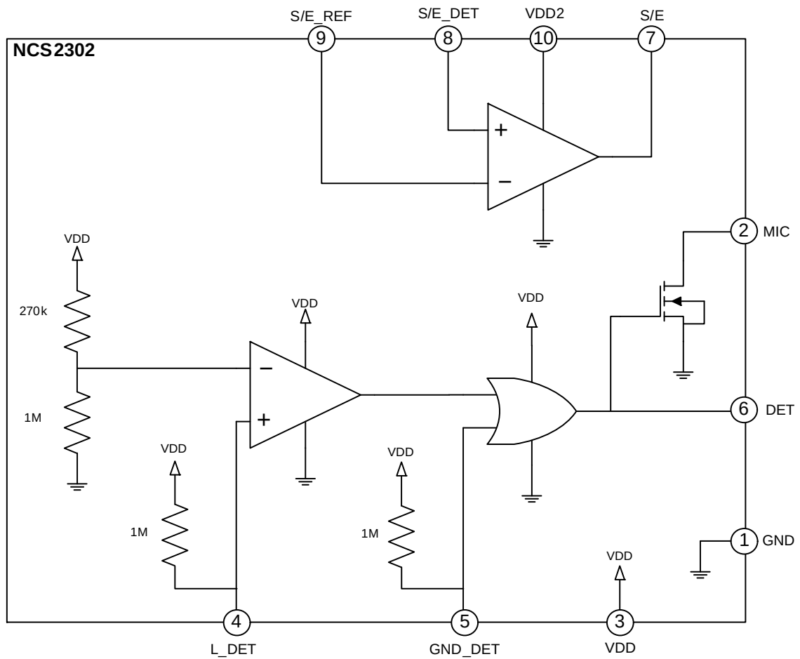
Figure 2. Block Diagram
