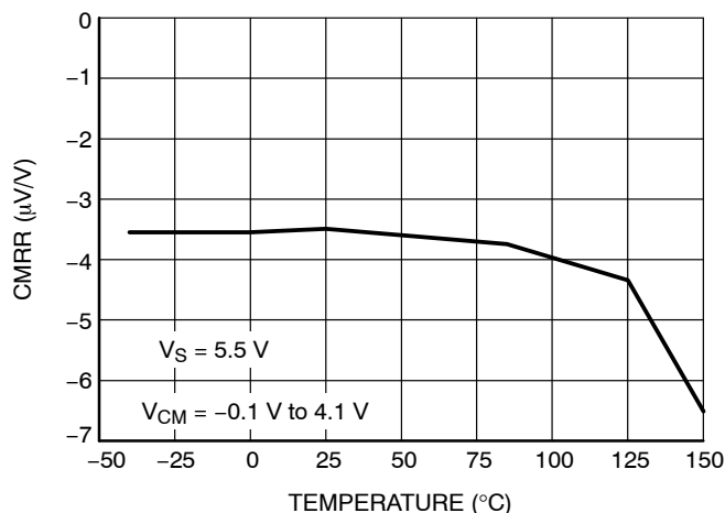
Figure 16. CMRR vs Temperature
