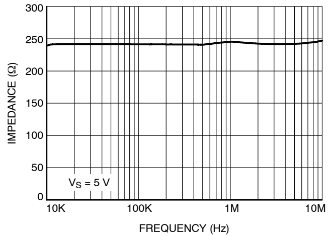
Figure 33. Open Loop Output Impedance vs. Frequency
