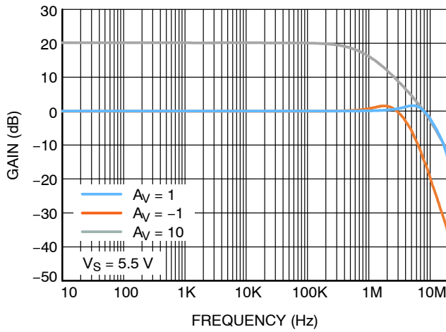
Figure 10. Closed Loop Gain vs. Frequency
