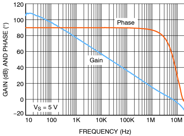
Figure 8. Open Loop Gain vs. Frequency
