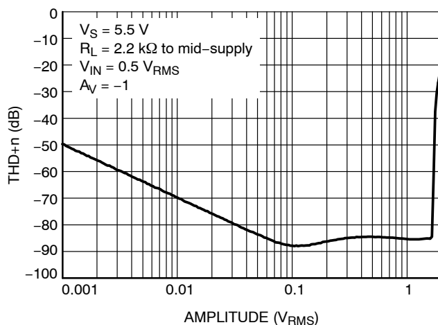
Figure 21. THD+n vs. Output Amplitude
