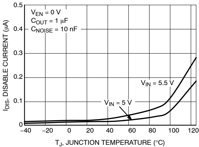
Figure 13. Disable Ground Pin Current vs. Temperature
