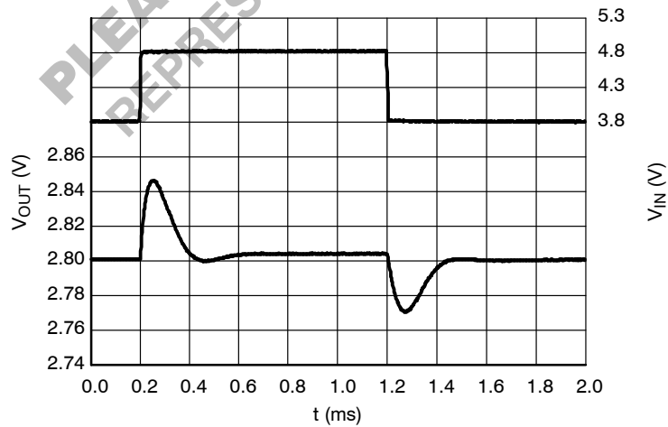
Figure 24. Line Transients, 2.8 V Version, t_R = t_F = 5 \mu s , I_{OUT} = 1 \text{ mA} , AE = 0 \text{ V}
