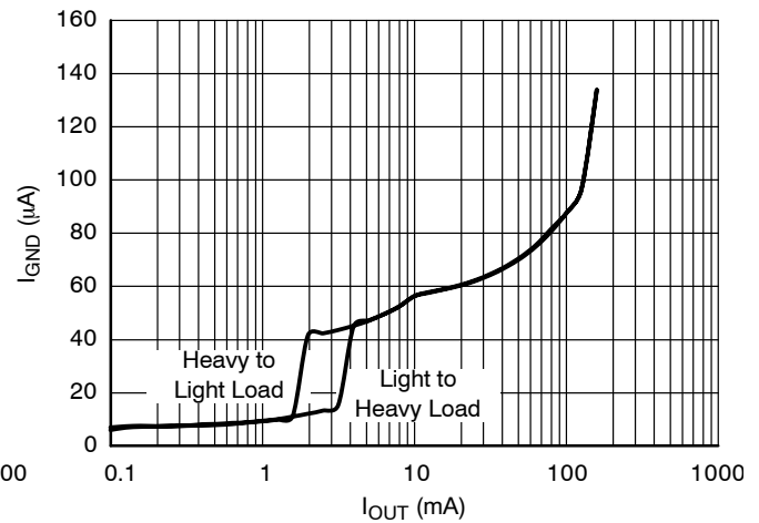
Figure 14. Supply Current vs. Output Current, 2.8 V Version, V_{IN} = 3.8\text{ V} , V_{AE} = 0\text{ V}
