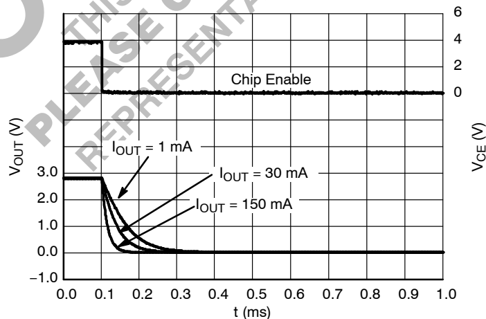
Figure 42. Shutdown, 2.8 V Version, V_{IN} = 3.8 V
