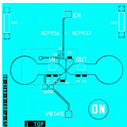
Figure 7. PCB Top View
