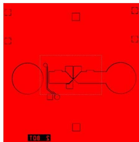
Figure 8. PCB Bottom View
