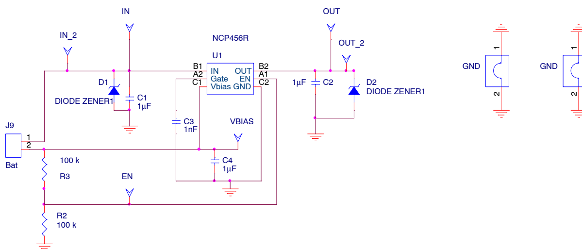
Figure 9. Board Schematic
