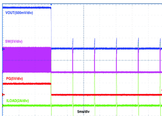
Figure 10. Over Current Protection, Hiccup Mode
