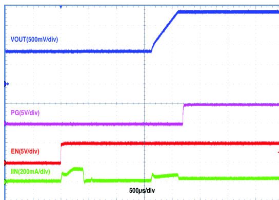
Figure 8. Start-up With 50% Pre-bias
