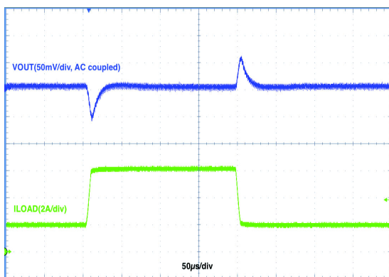
Figure 9. Load Transient, 2 A <-> 6 A, Slew Rate = 1 A/µs
