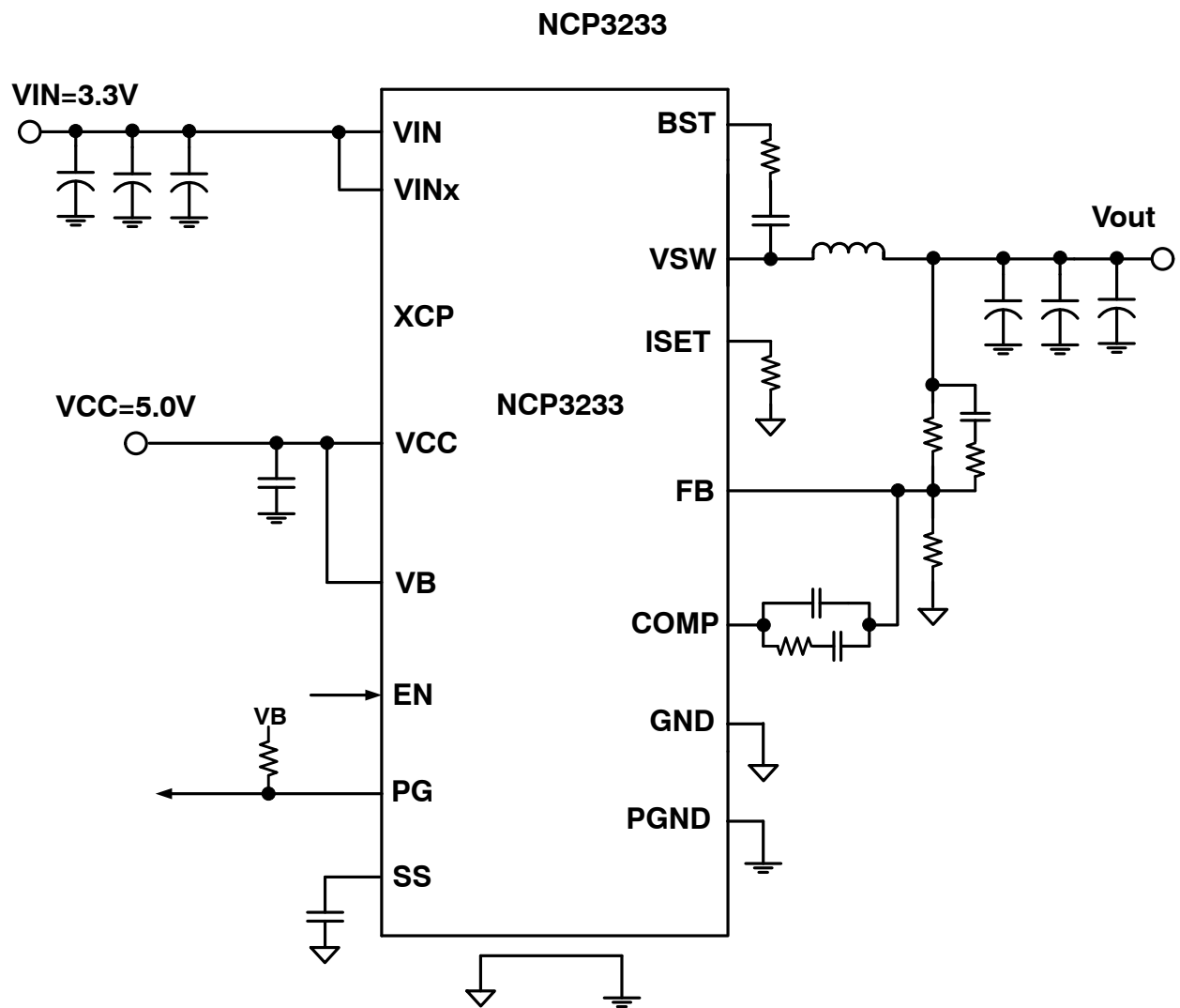
Figure 3. Typical Application Circuit for Separate Rail in System V_{IN} = 3.3V and V_{CC} = 5V
