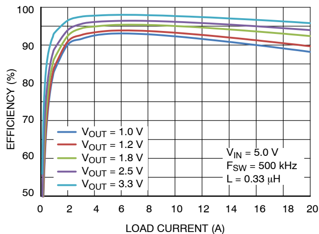
Figure 7. Efficiency vs. Load Current ( V_{IN} = 5.0 V), Inductor: Würth Electronics 7443320033
