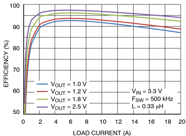
Figure 6. Efficiency vs. Load Current ( V_{IN} = 3.3 V), Inductor: Würth Electronics 7443320033
