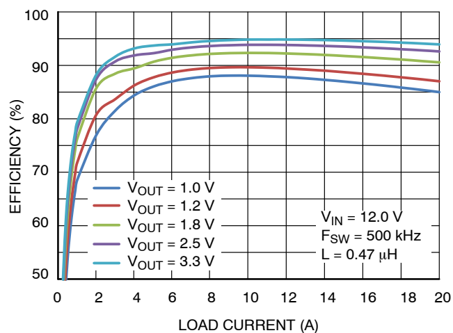
Figure 8. Efficiency vs. Load Current ( V_{IN} = 12.0 V), Inductor: Würth Electronics 7443320047
