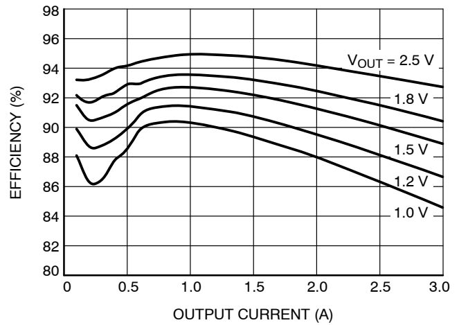
Figure 5. Efficiency at Auto CCM/DCM Mode V_{in} = 5.0\text{ V}
