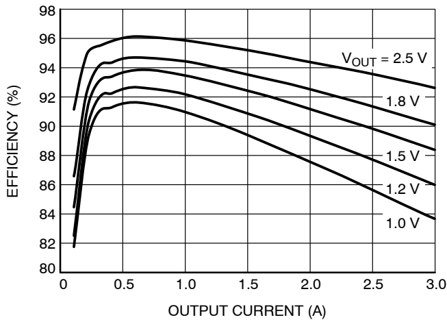
Figure 6. Efficiency at FCCM Mode V_{in} = 3.3\text{ V}
