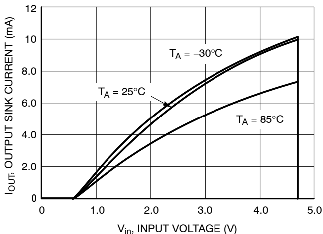
Figure 6. NCP304AH Series 4.5 V Reset Output Sink Current vs. Input Voltage
