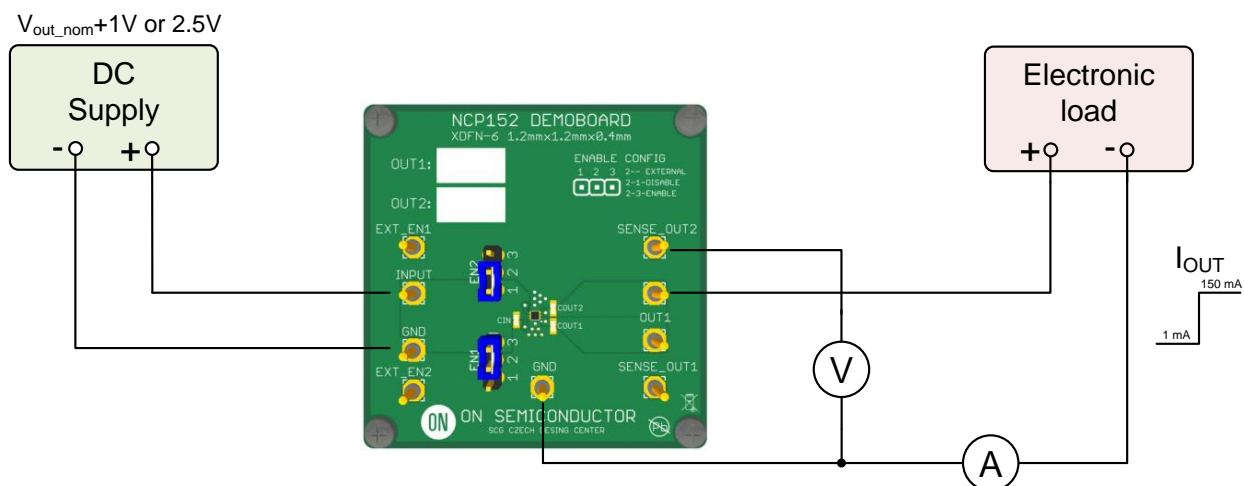
Figure 2: Test configuration for measurement REG_{LOAD} , Load Regulation
