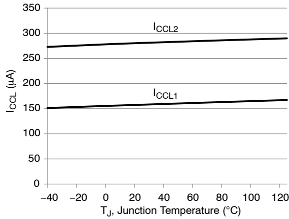
Figure 42. I CCL vs. Temperature
