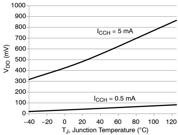
Figure 44. V DO vs. Temperature
