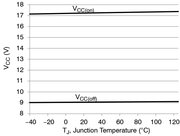
Figure 40. V CC(on/off) vs. Temperature
