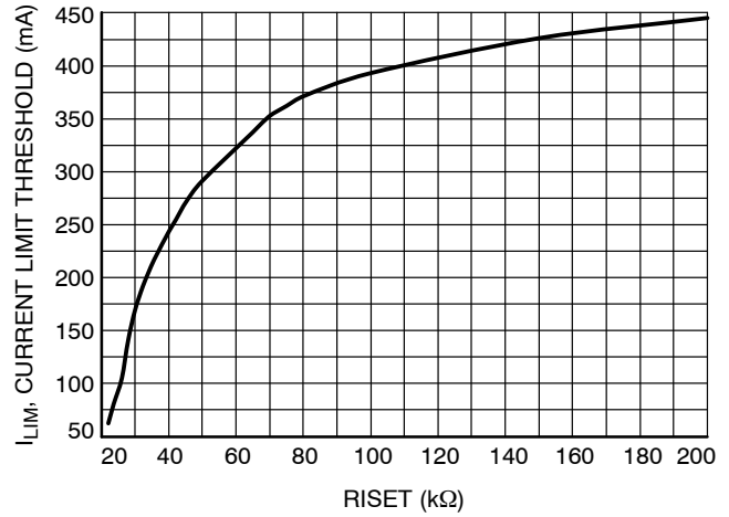
Figure 30. Current Limit Threshold vs. R_{CL} , Current Slew Rate = 0.5 A/ \mu\text{s}
