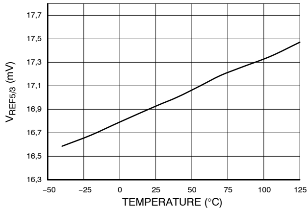
Figure 33. V REF5/3 vs. Temperature
