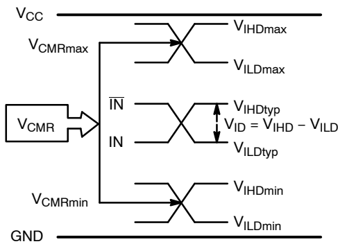
Figure 10. V_{CM} Diagram
