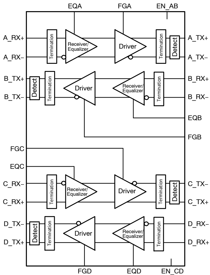
Figure 1. Logic Diagram of NB7NPQ1204M
