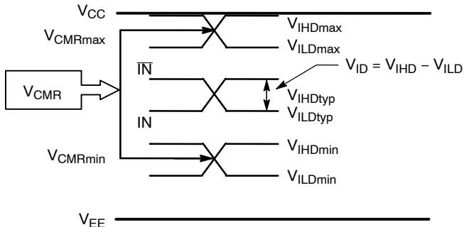
Figure 5. V_{th} Diagram
