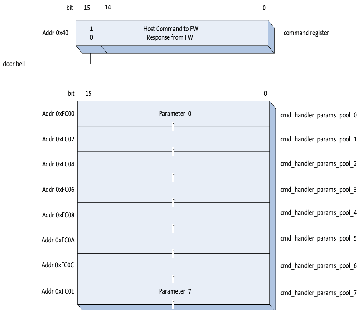
Figure 21: Interface Structure
