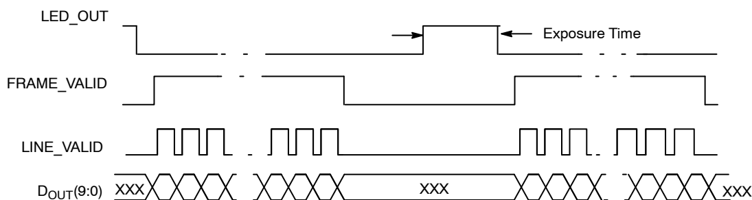
Figure 15. Sequential Master Mode Synchronization Waveforms
