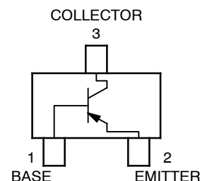
SC-70 (SOT-323) CASE 419 STYLE 3
