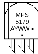
TO-92 CASE 29-11 STYLE 1
