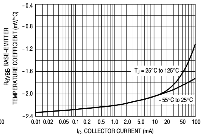
Figure 9. Temperature Coefficients
