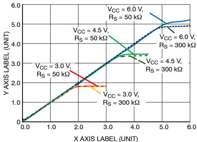
Figure 10. Offset Voltage at Demodulator Output as a Function of V_{COin} and R_S
