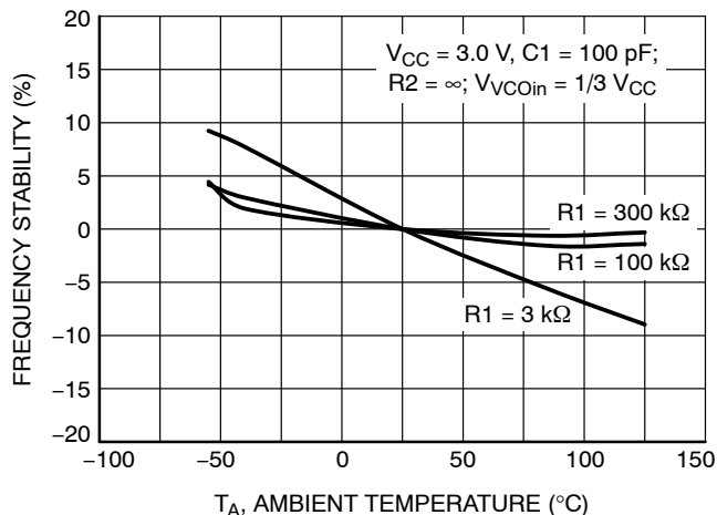
Figure 11A. Frequency Stability vs. Ambient Temperature: V_{CC} = 3.0\text{ V}
