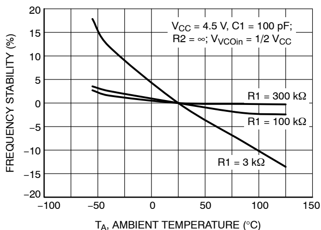
Figure 11B. Frequency Stability vs. Ambient Temperature: V_{CC} = 4.5\text{ V}
