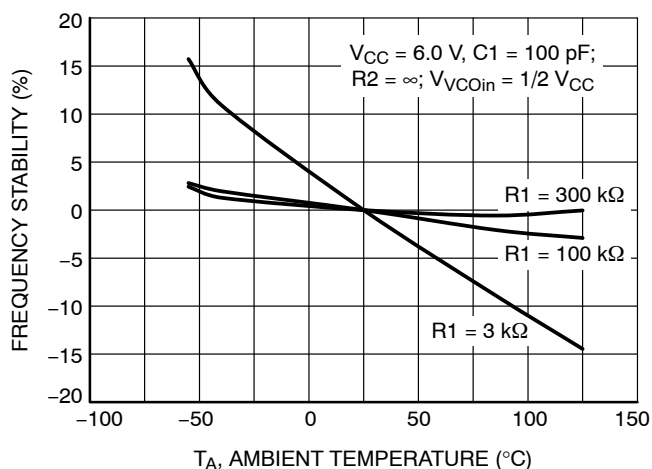
Figure 11C. Frequency Stability vs. Ambient Temperature: V_{CC} = 6.0\text{ V}
