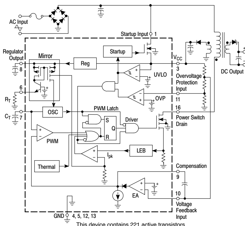
Figure 1. Simplified Application
