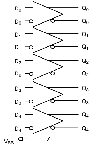
Figure 2. Logic Diagram
