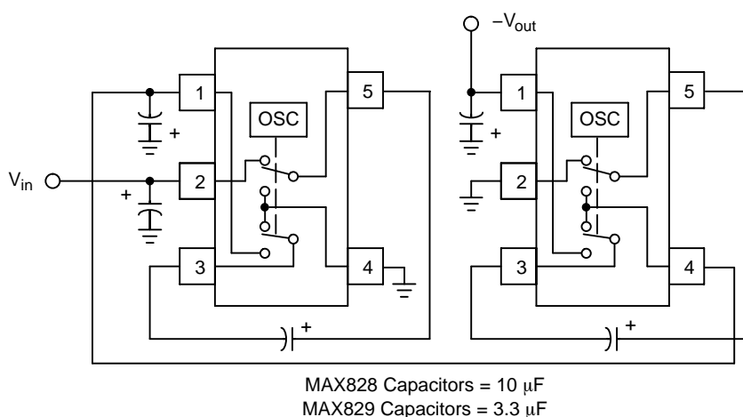
Figure 27. Cascade Devices for Increased Negative Output Voltage
