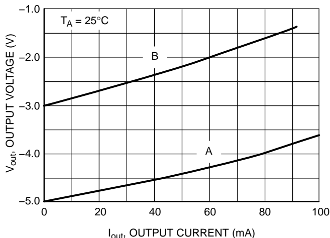
Figure 43. Parallel Load Regulation, Output Voltage vs. Output Current MAX828
