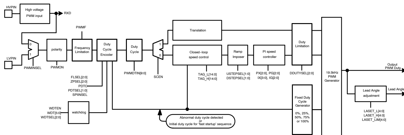
Figure 14. PWM Command Flow and Related Registers
