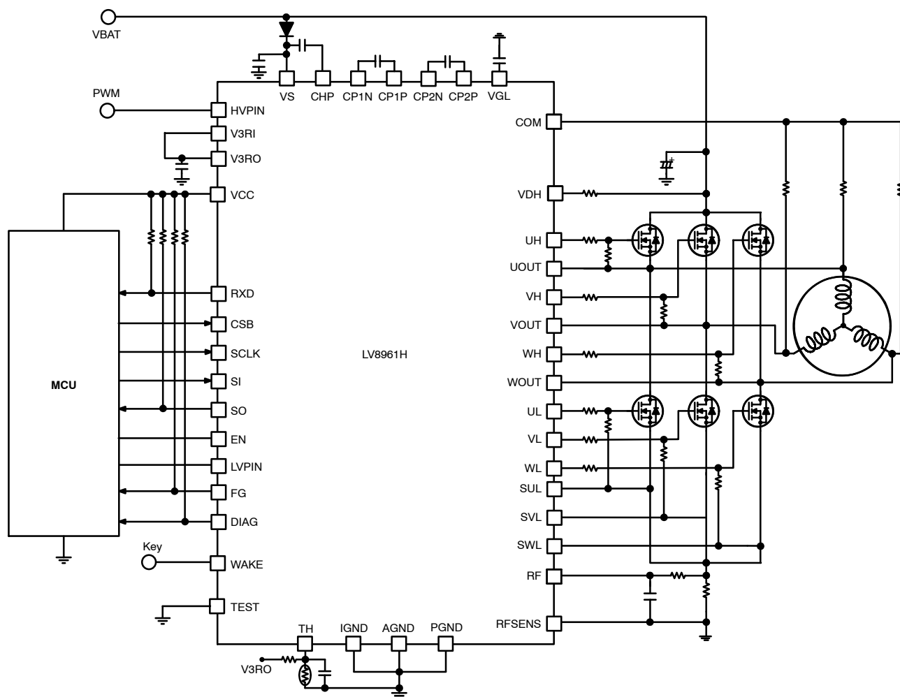
Figure 3. Example of MCU Based Control Configuration
