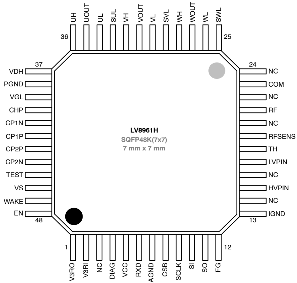
Figure 4. LV8961H Pinout
