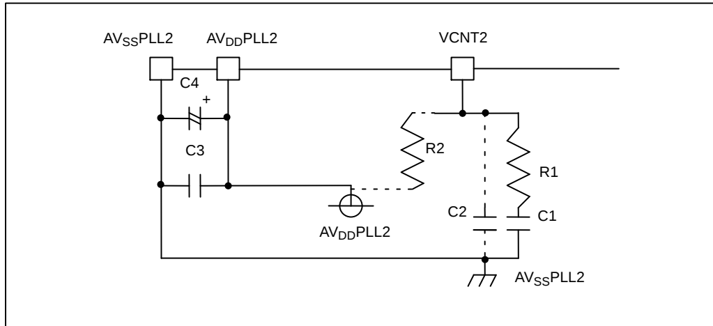
Figure 41. PLL2 (Audio)
