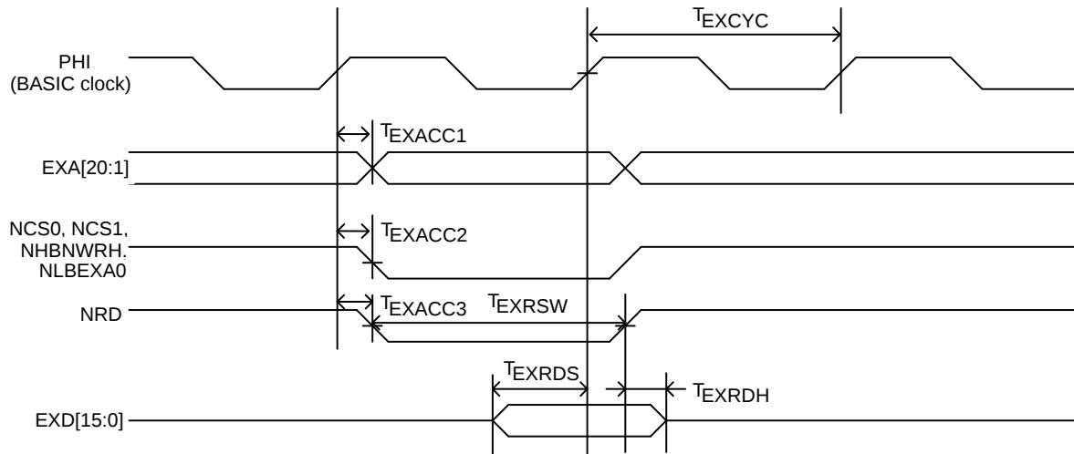
Figure 17. AC Characteristics – External Memory Bus Read Timing
