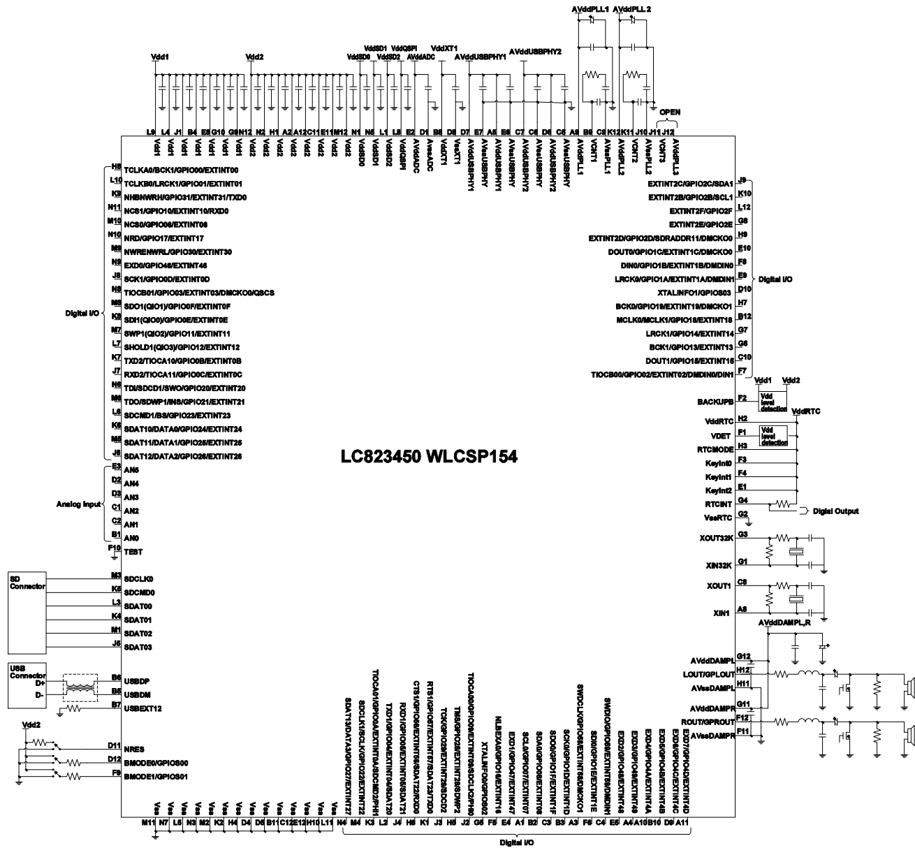
Figure 55. Application Diagram
