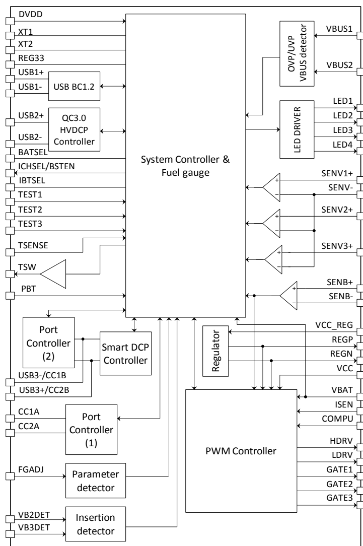
Figure 2: Block diagram
