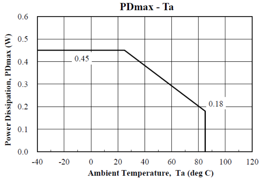
Pdmax-Ta Graph
