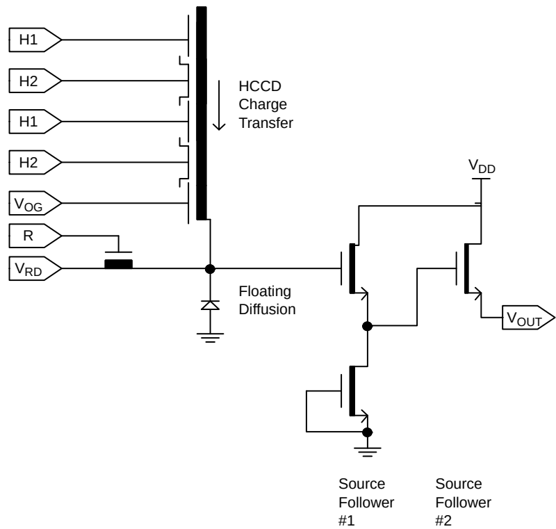
Figure 4. Output Schematic
