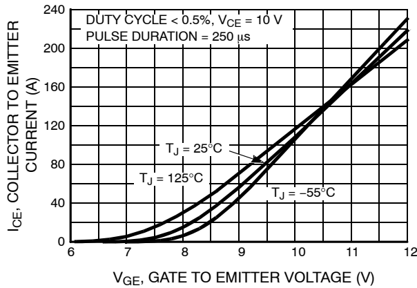
Figure 13. TRANSFER CHARACTERISTIC
