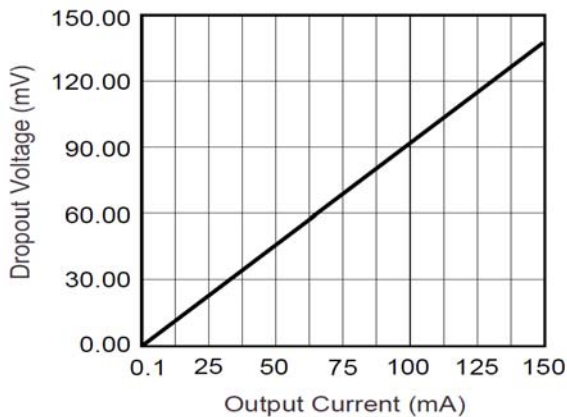
Figure 19. Dropout Voltage
