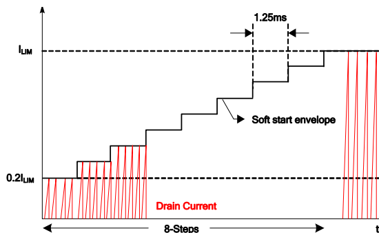
Figure 27. Internal Soft-Start
