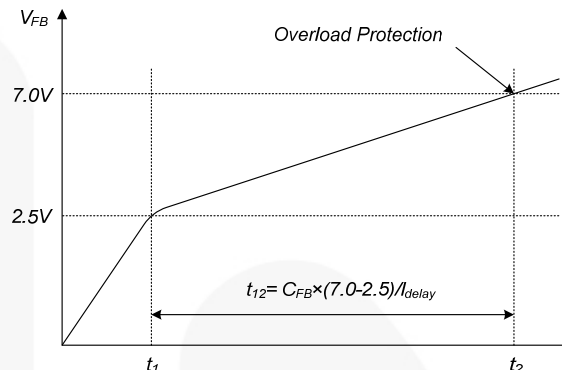
Figure 20. Overload Protection
