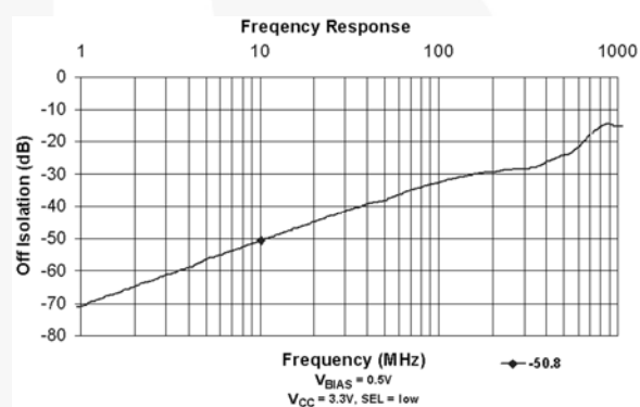
Figure 7. Off Isolation
