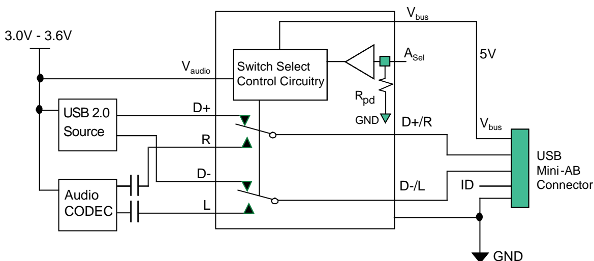
Figure 5. Typical Application
