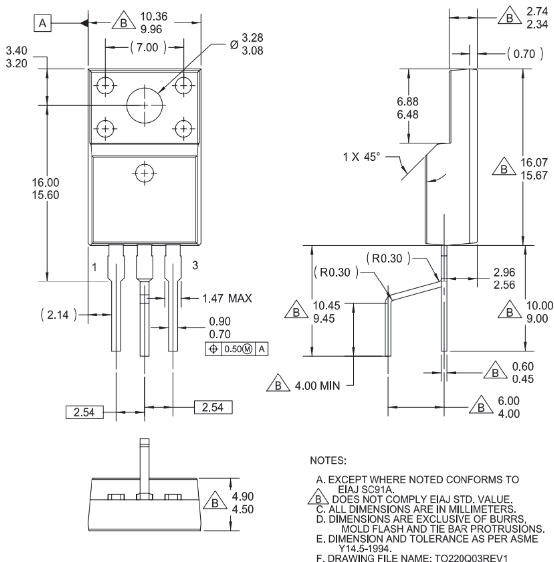
Figure 18. TO220, Molded, 3-Lead, Full Pack, EIAJ SC91, Y-Formed
