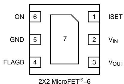
Figure 3. Pin Configuration
