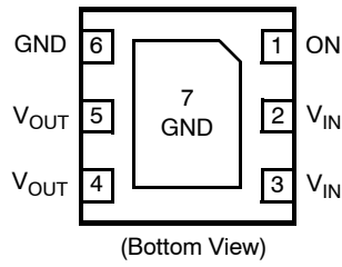
Figure 3. Pin Configuration
