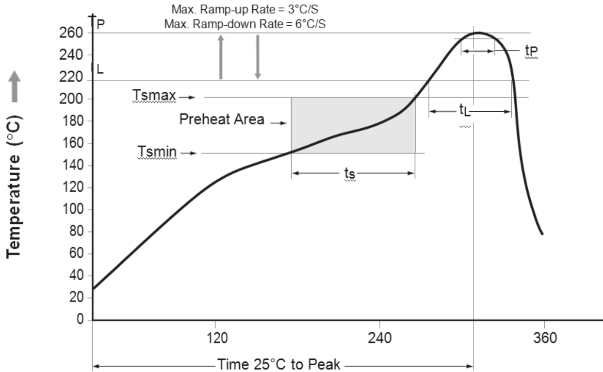
Figure 12. Reflow Profile
