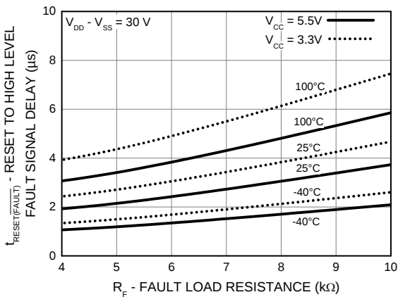
Figure 27. RESET to High Level Fault Signal Delay ( t_{\text{RESET}(\text{FAULT})} ) vs. Fault Load Resistance ( R_F )
