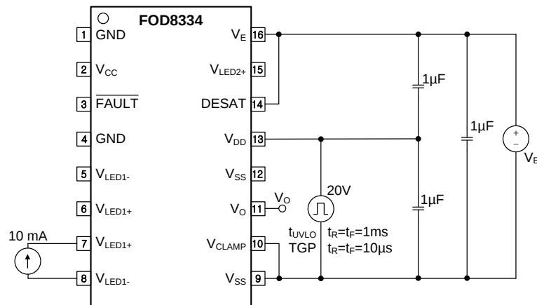
Figure 49. Under-Voltage Lockout Delay ( t_{UVLO} ), Time to Good Power Delay ( t_{GTP} ) Test Circuit
