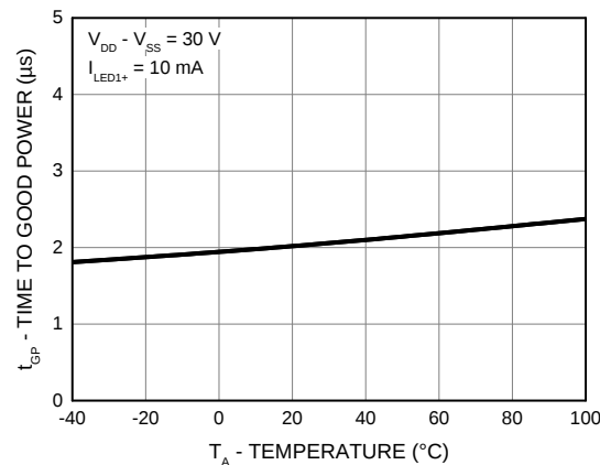
Figure 28. Time to Good Power ( t_{\text{GP}} ) vs. Temperature
