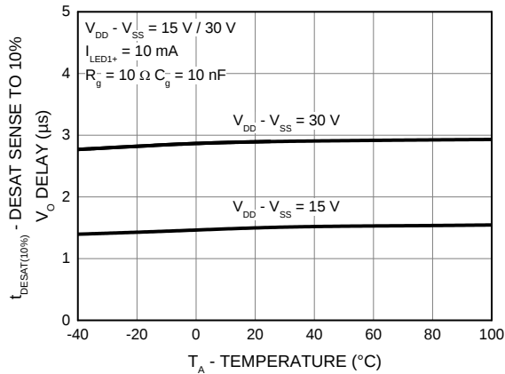
Figure 23. DESAT Sense to 10% V_O Delay ( t_{\text{DESAT}(10\%)} ) vs. Temperature
