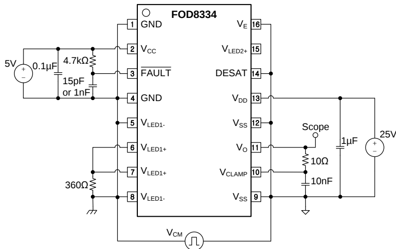
Figure 50. Common-Mode Low (CML) LED1-Off Test Circuit
