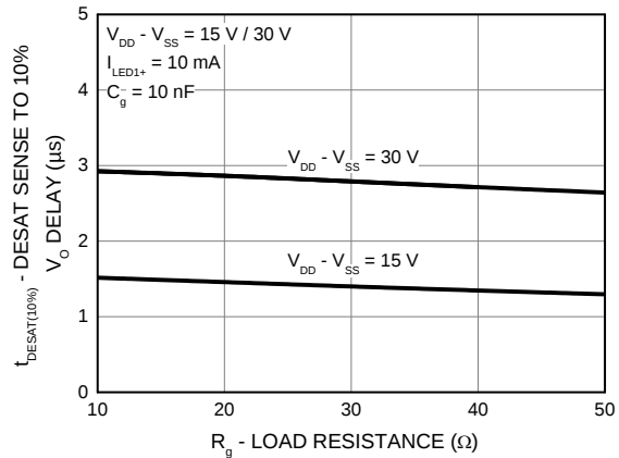
Figure 24. DESAT Sense to 10% V_O Delay ( t_{\text{DESAT}(10\%)} ) vs. Load Resistance ( R_g )
