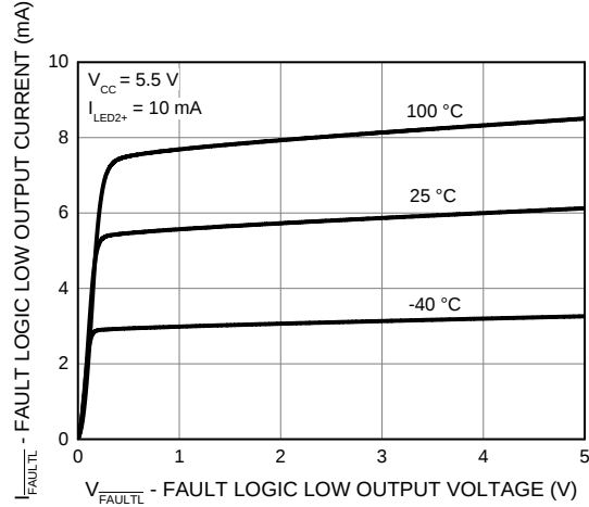
Figure 17. FAULT Logic Low Output Current ( I_{\text{FAULTL}} ) vs. Voltage ( V_{\text{FAULTL}} )
