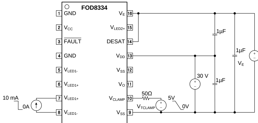
Figure 41. Clamping Threshold Voltage ( V_{CLAMP\_THRES} ) Test Circuit
