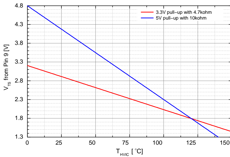
Figure 6. V-T Curve of Temperature Output of IC
